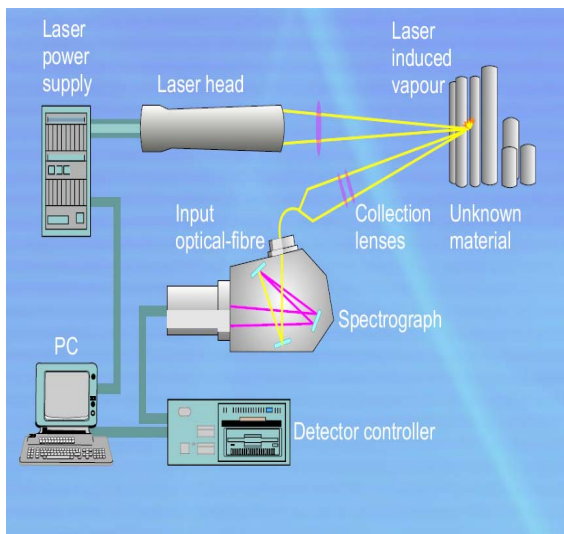
FIG. 6. LIBS comprises (i) a laser system to ablate the material surface to create a micro-plasma, and (ii) a spectrometer to generate a spectroscopic profile of the micro-plasma's constituent components.
