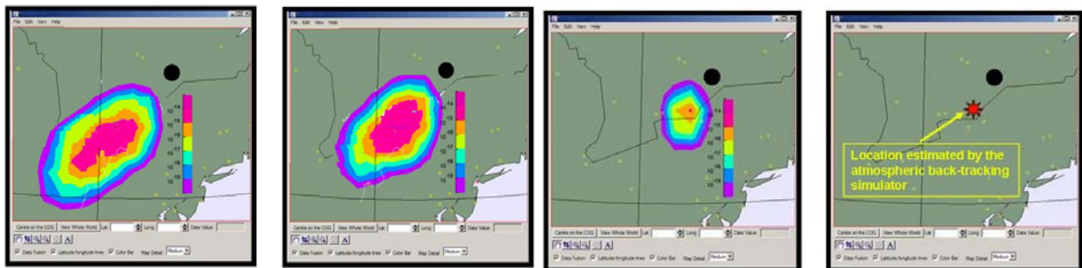
FIG. 11. Airborne material is identified through sample analysis, and the data are combined with meteorological information in a suitable atmospheric computer model to provide an estimate of the source direction and probable location.
