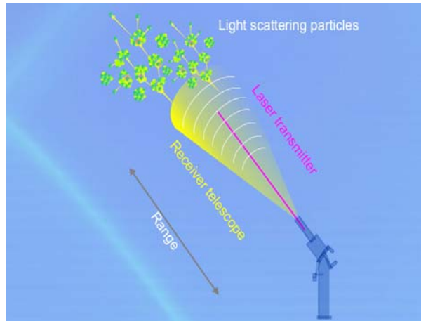
FIG. 8. LIDAR methods are used routinely by environmental monitoring agencies to determine the presence of pollutants in the atmosphere.
