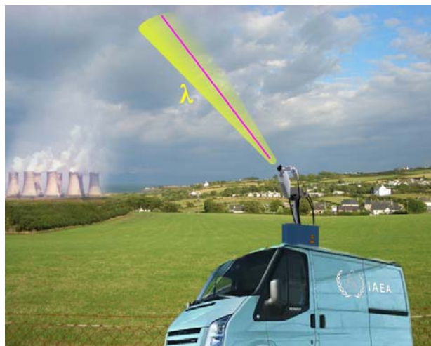
FIG. 9. A mobile LIDAR travels to the vicinity of a suspected location engaged in undeclared NFC processes. A laser, tunable to precise wavelengths ( \lambda ) selectively stimulates specific airborne molecules emanating as gaseous compound from the process. A light-sensitive telescope scans the atmosphere, detecting the presence of the stimulated molecules.
